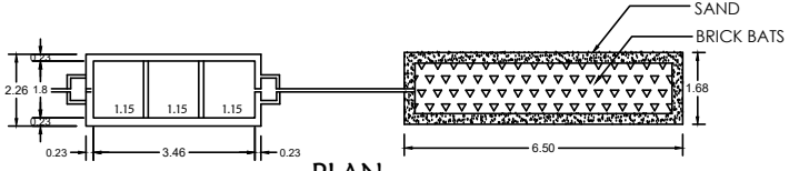
PLAN SEPTIC TANK AND TRENCH
