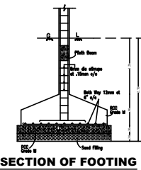
SECTION OF FOOTING
