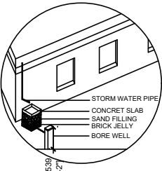
RAINWATER HARVESTING
