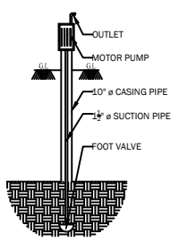
SECTION OF BOREWELL
