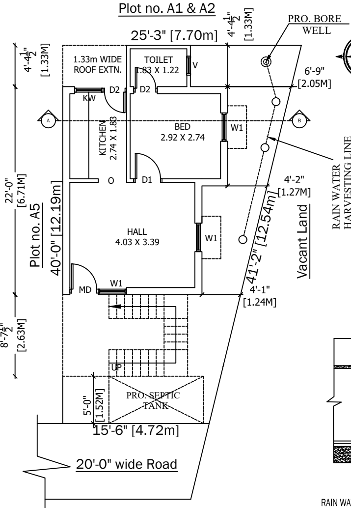
SITE CUM PRO. GROUND FLOOR PLAN SCALE : 1:100
