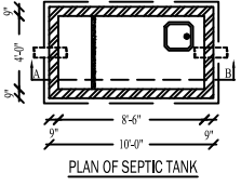
PLAN OF SEPTIC TANK
