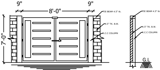
ELEVATION & SECTION OF COMPOUND WALL & MAIN GATE
