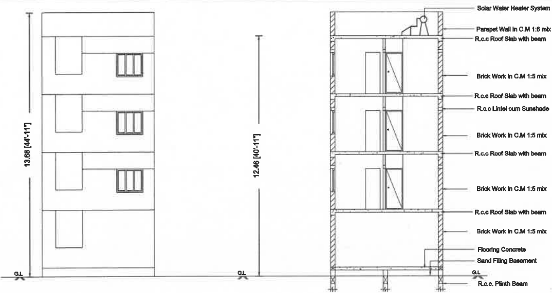
FRONT ELEVATION
