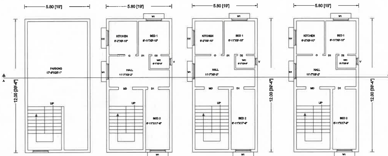
STILT FLOOR
