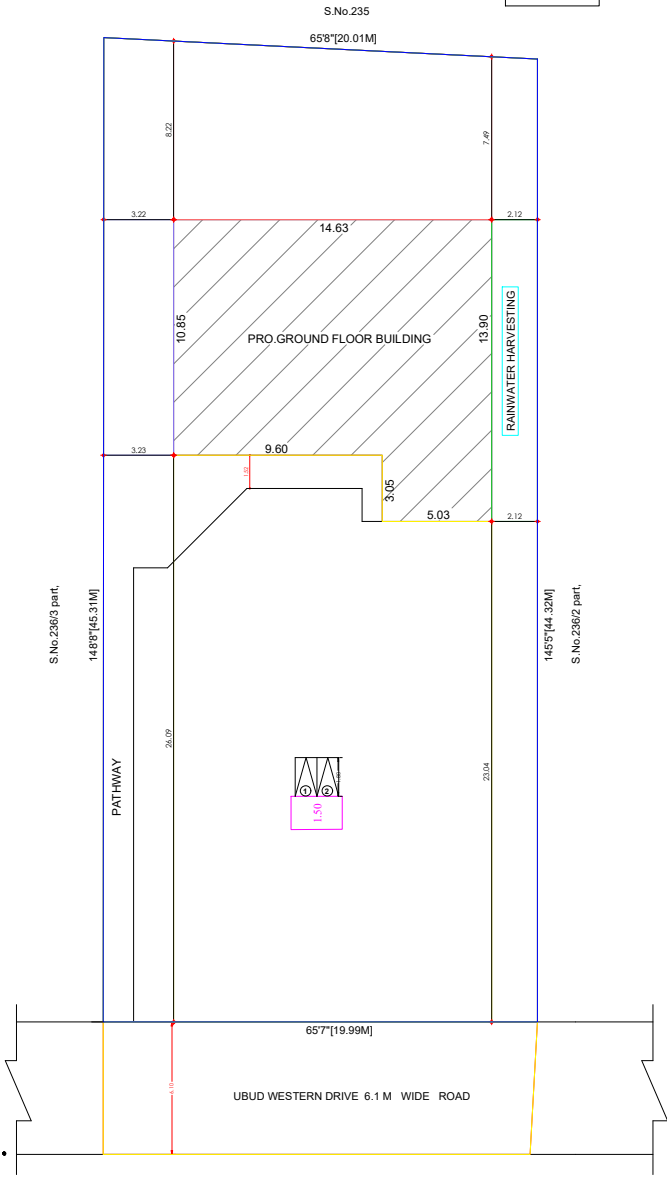
SITE PLAN
