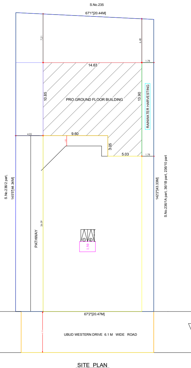
SITE PLAN
