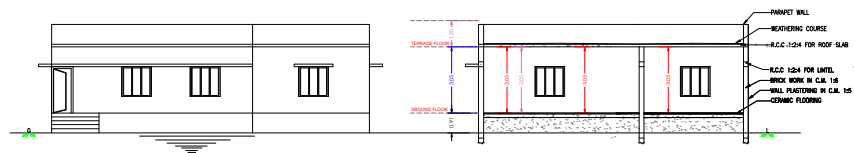
SECTION ON "AB"
