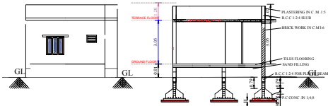
SECTION 'SC'
