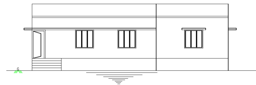
FROUNT ELEVATION
