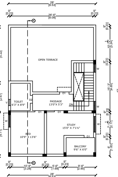
PRO.SECOND FLOOR(PT) PLAN
