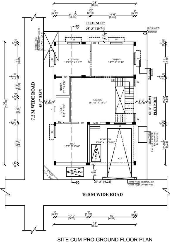
SITE CUM PRO.GROUND FLOOR PLAN
