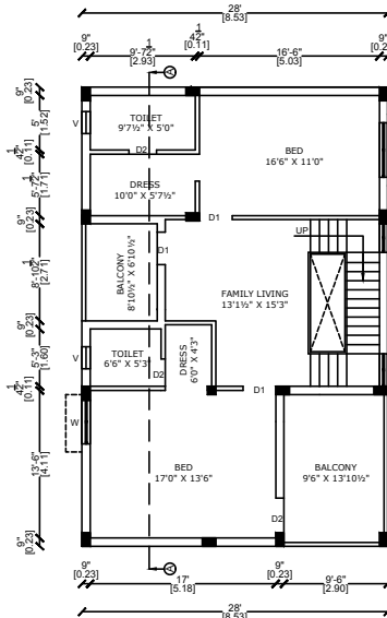
PRO.FIRST FLOOR PLAN
