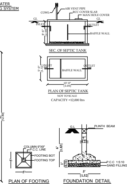
PLAN OF FOOTING
