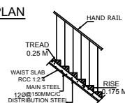
STAIR CASE DETAILS SCALE 1:300
