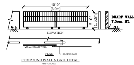
COMPOUND WALL & GATE DETAIL NOT TO SCALE
