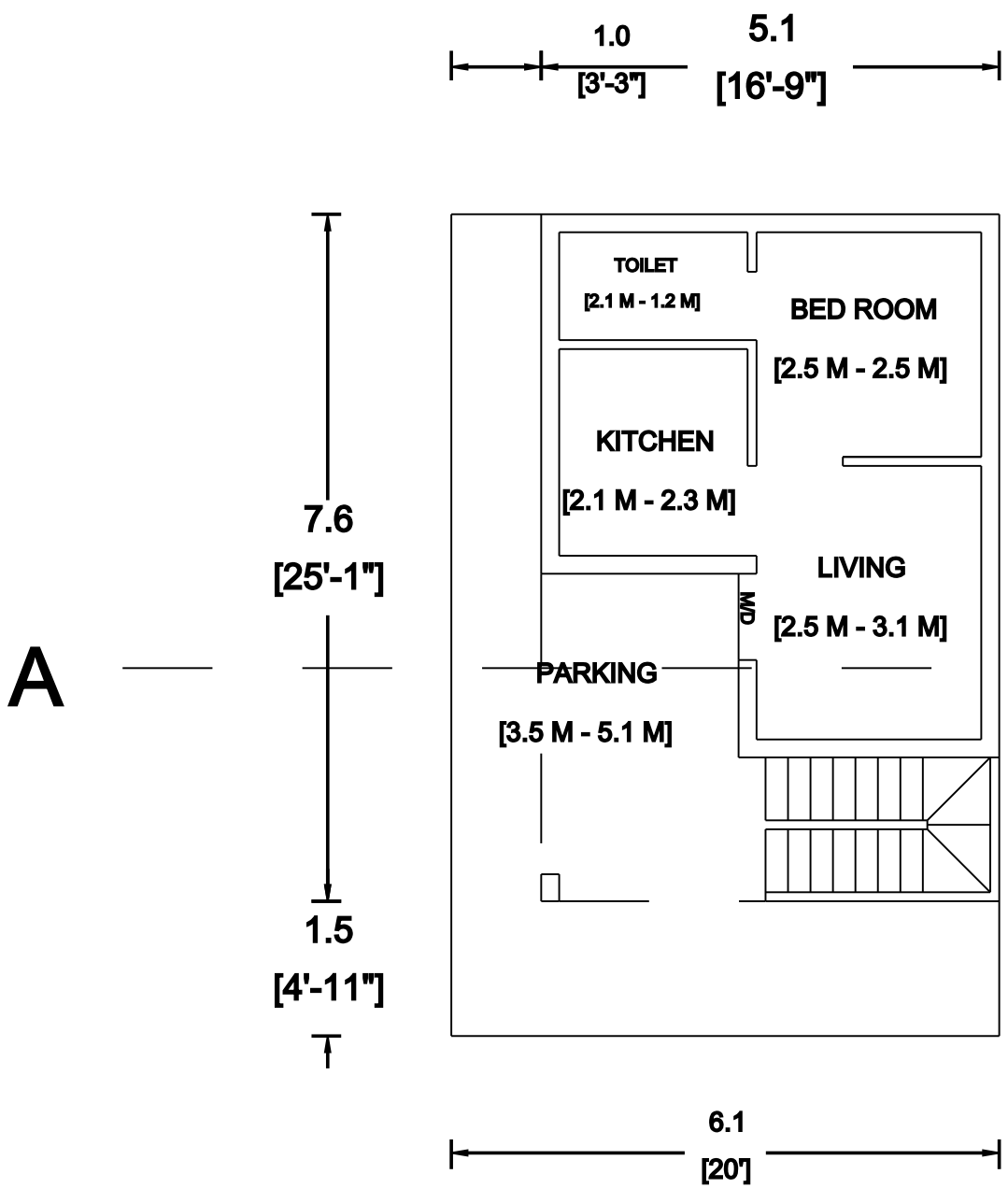
GROUND FLOOR
