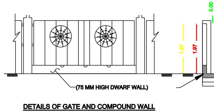
DETAILS OF GATE AND COMPOUND WALL
