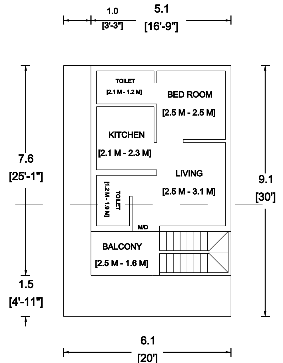
FIRST FLOOR
