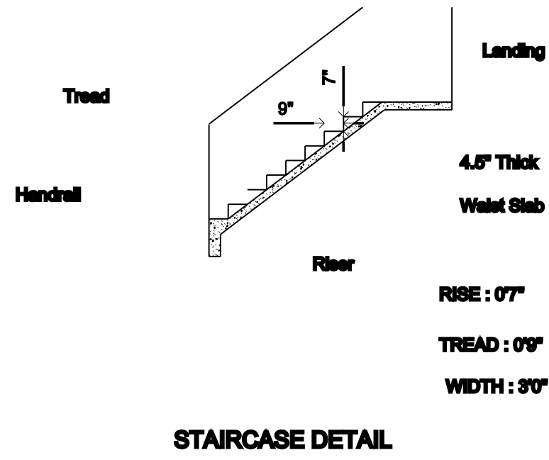
STAIRCASE DETAIL
