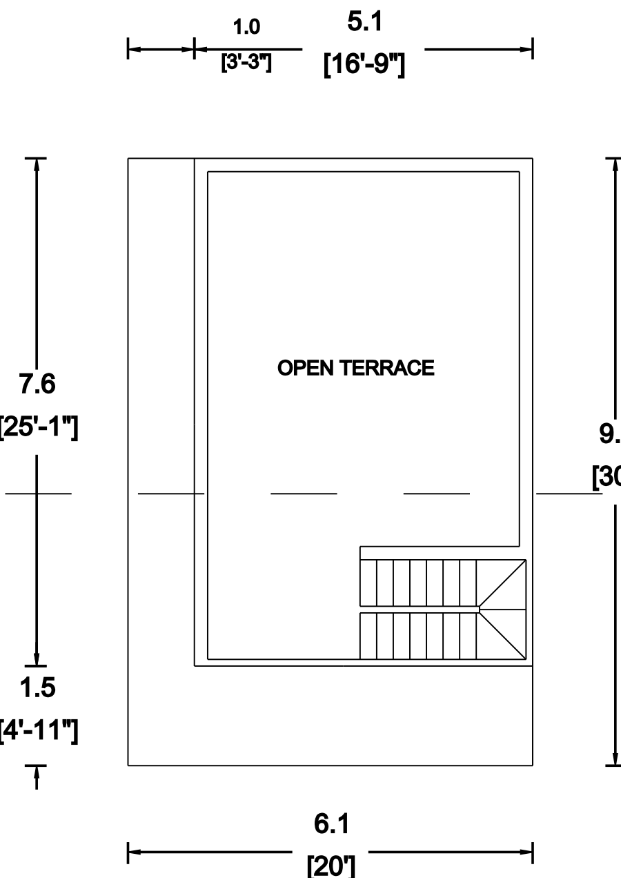
TERRACE PLAN
