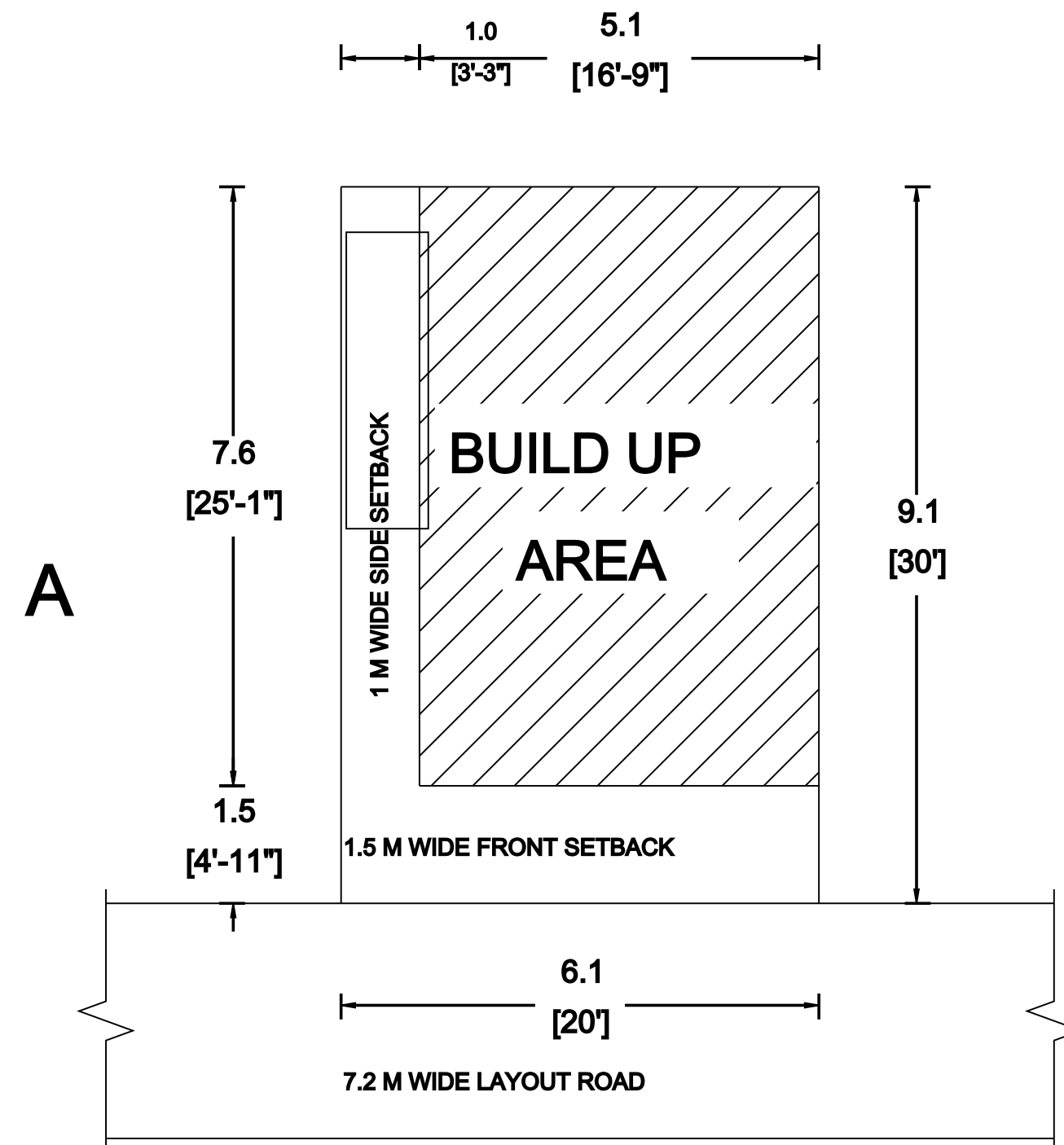
SITE CUM PROPOSED
