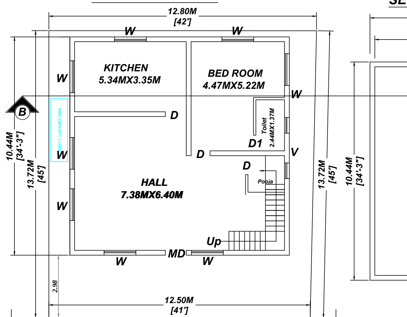
SITE PLAN CUM GROUND FLOOR PLAN
