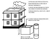
STORAGE DETAILS
