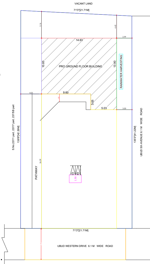
SITE PLAN
