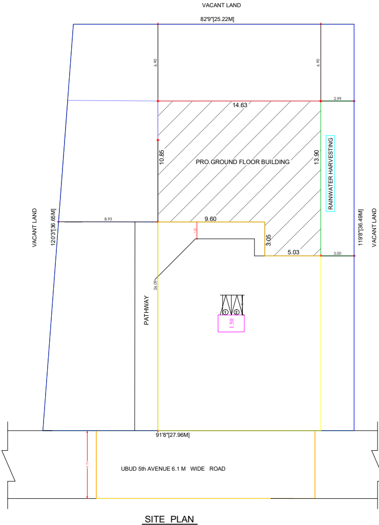
SITE PLAN
