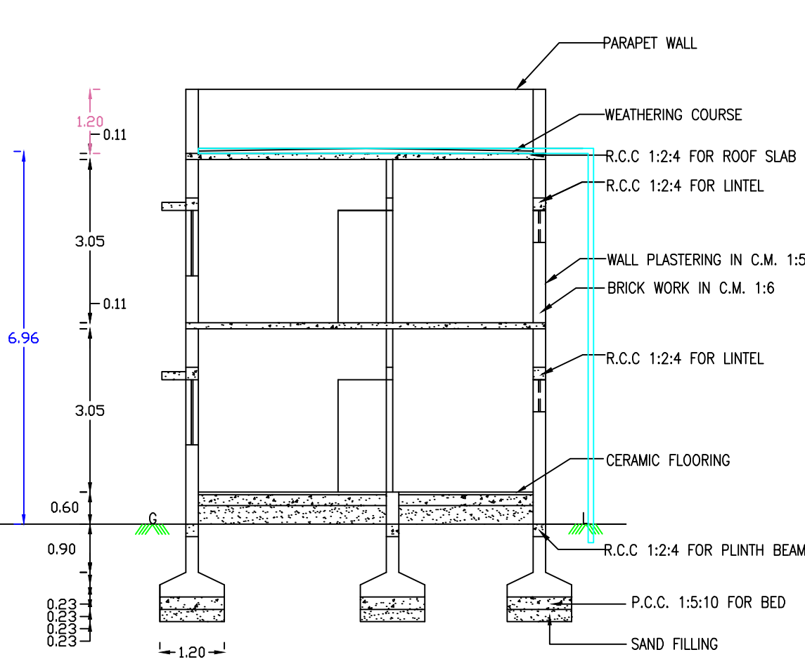
SECTION ON "RC"
