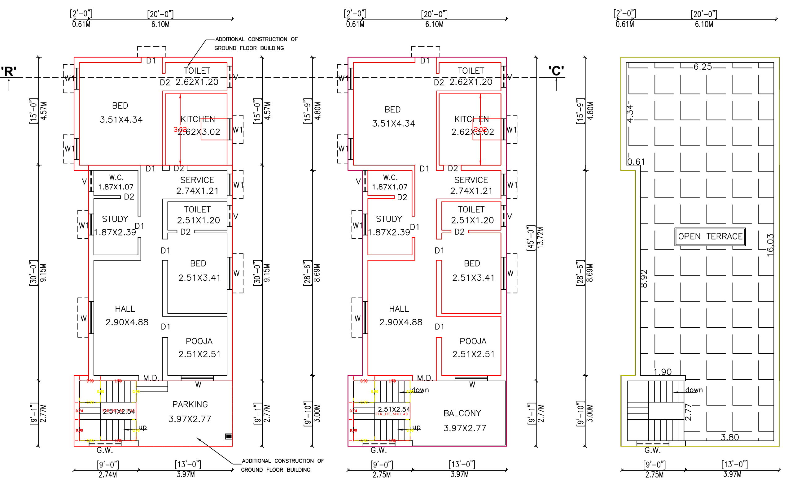
EXISTING & PROPOSED GROUND FLOOR PLAN
