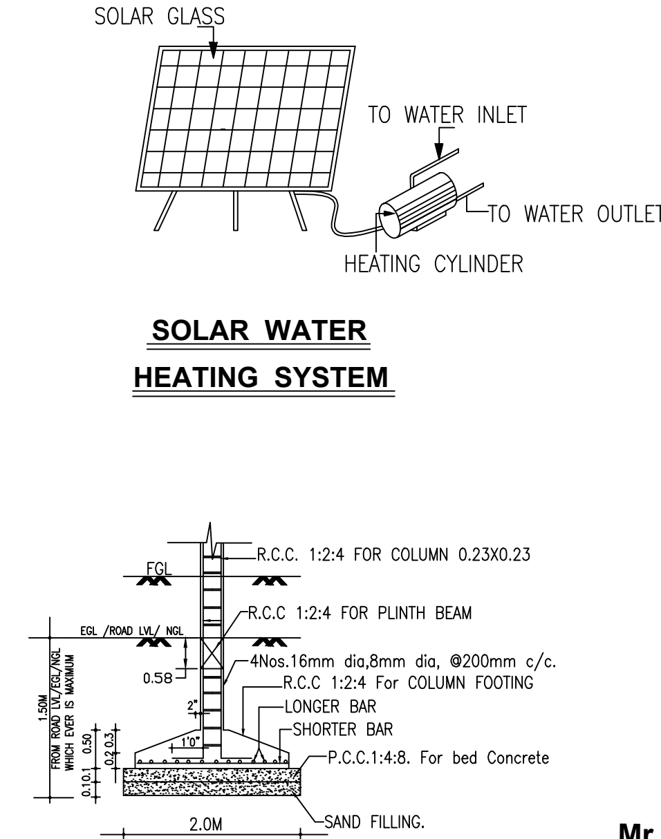
FOUNDATION DETAILS
