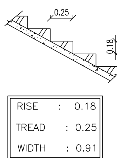
STAIRS DETAILS
