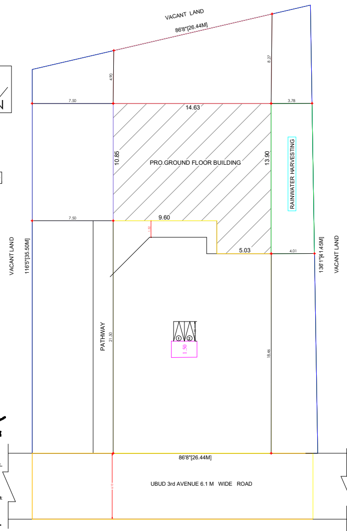
SITE PLAN
