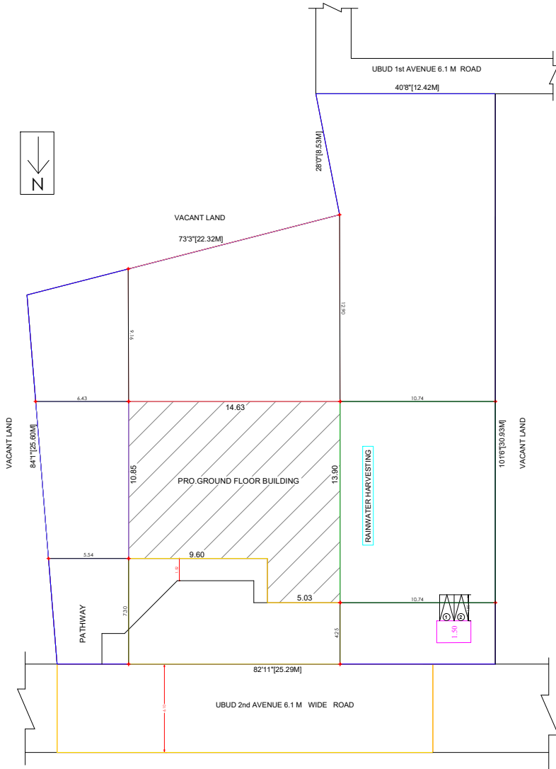
SITE PLAN
