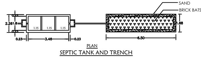
SEPTIC TANK AND TRENCH
