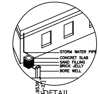
RAINWATER HARVESTING
