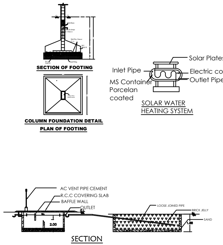
SECTION
