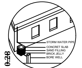
DETAIL RAINWATER HARVESTING
