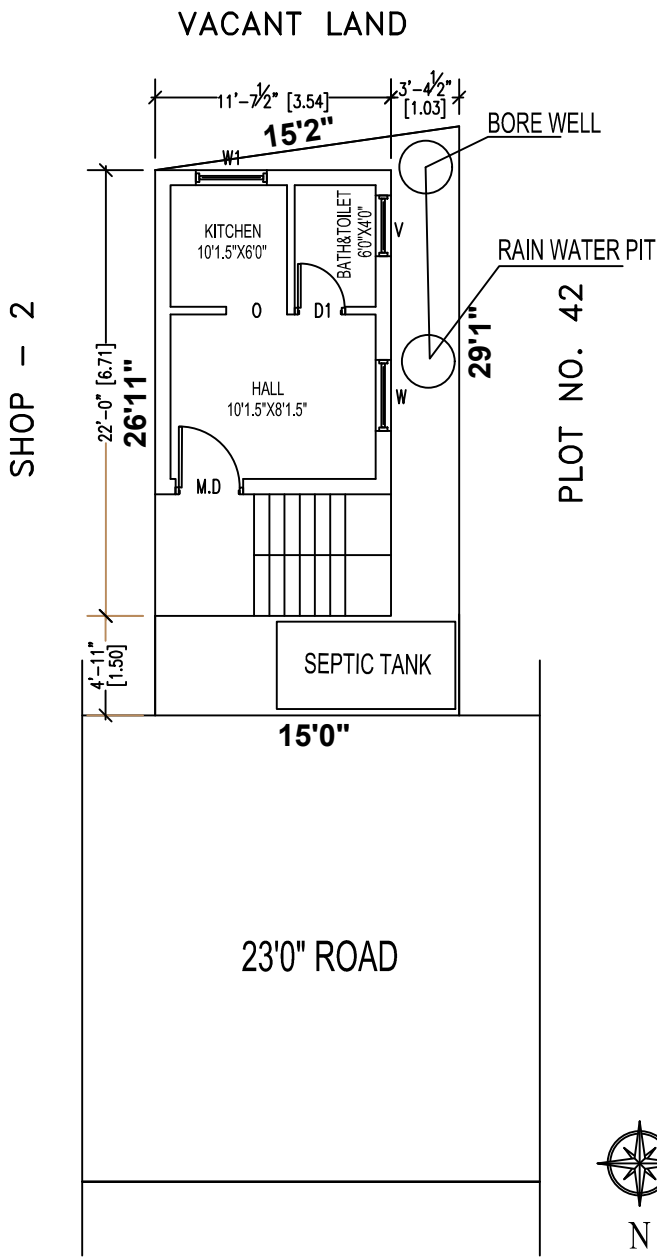
SITE CUM GROUND FLOOR PLAN
