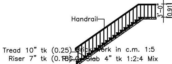
Staircase Details
