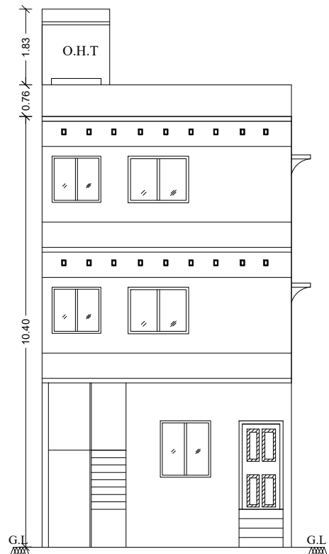
FRONT ELEVATION
