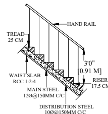
STAIR CASE PLAN (SCALE- 1:300)
