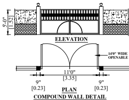
COMPOUND WALL DETAIL
