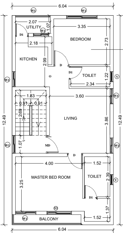
TYPICAL FIRST AND SECOND FLOOR PLAN
