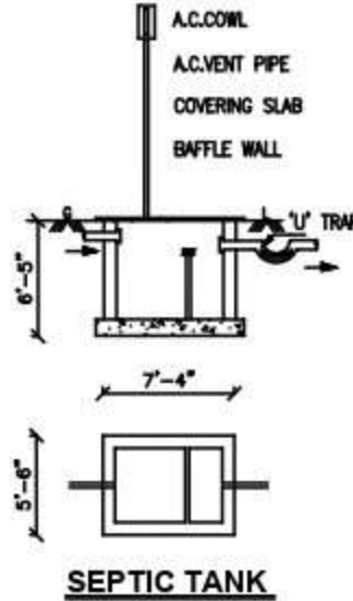
SEPTIC TANK
