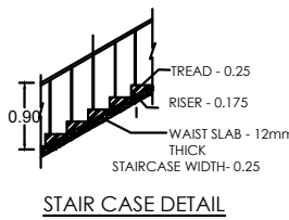
STAIR CASE DETAIL
