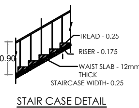
STAIR CASE DETAIL
