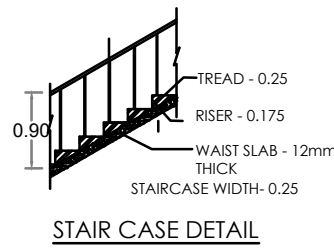
STAIR CASE DETAIL
