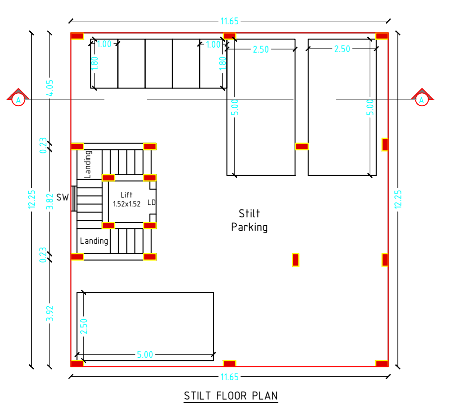
STILT FLOOR PLAN
