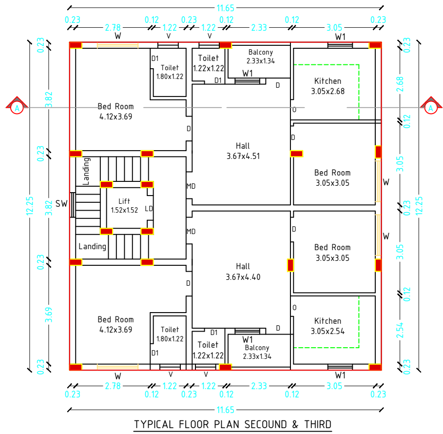
TYPICAL FLOOR PLAN SECOND & THIRD
