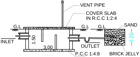
SECTION-AB
