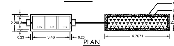
SEPTIC TANK AND TRENCH
