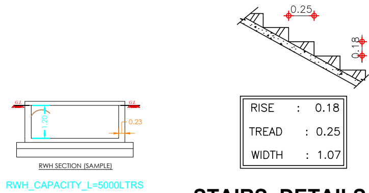
STAIRS DETAILS
