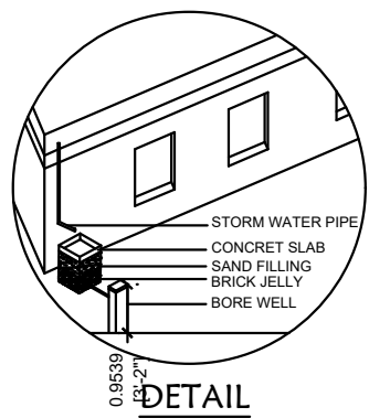
RAINWATER HARVESTING
