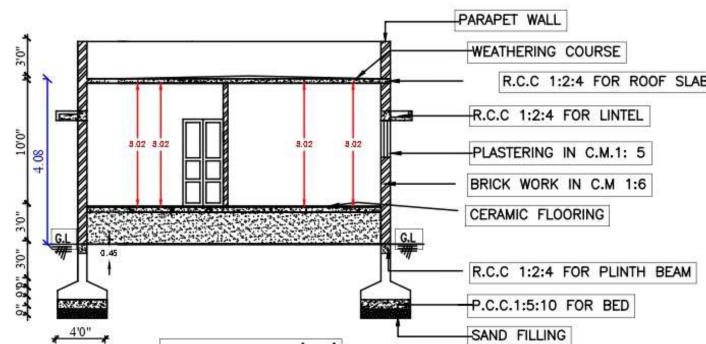
SECTION ON 'SC'
