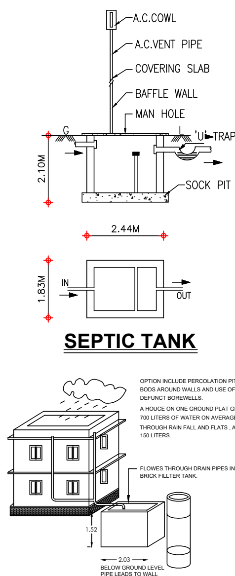
BORE (OR) WELL AND RAIN WATER STORAGE DETAILS
