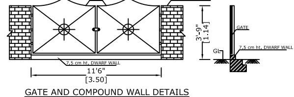
GATE AND COMPOUND WALL DETAILS
