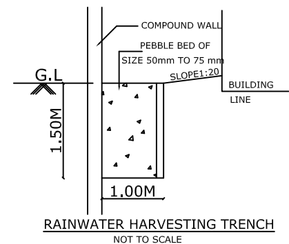
RAINWATER HARVESTING TRENCH
