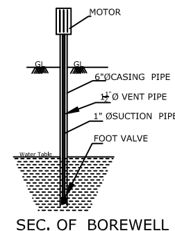
SEC. OF BOREWELL
