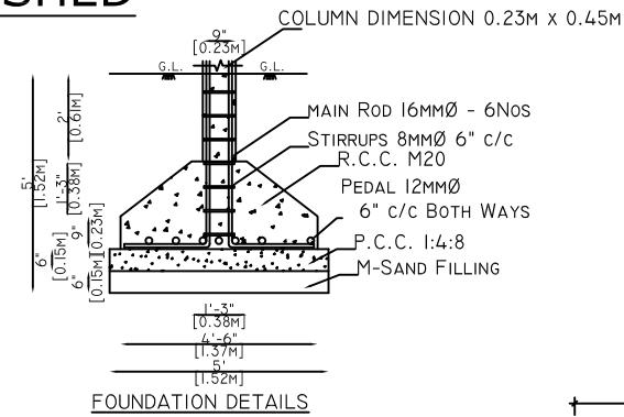
CONE CRUSHER SHED
