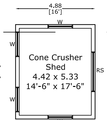
CONE CRUSHER SHED
