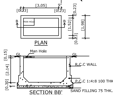
UG SUMP DETAIL
