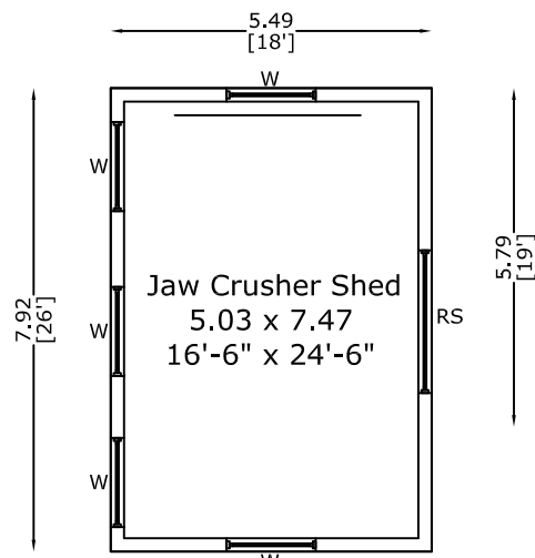
JAW CRUSHER SHED
