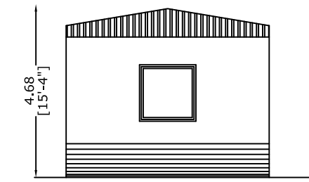
TYPICAL ELEVATION
