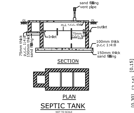
SEPTIC TANK
