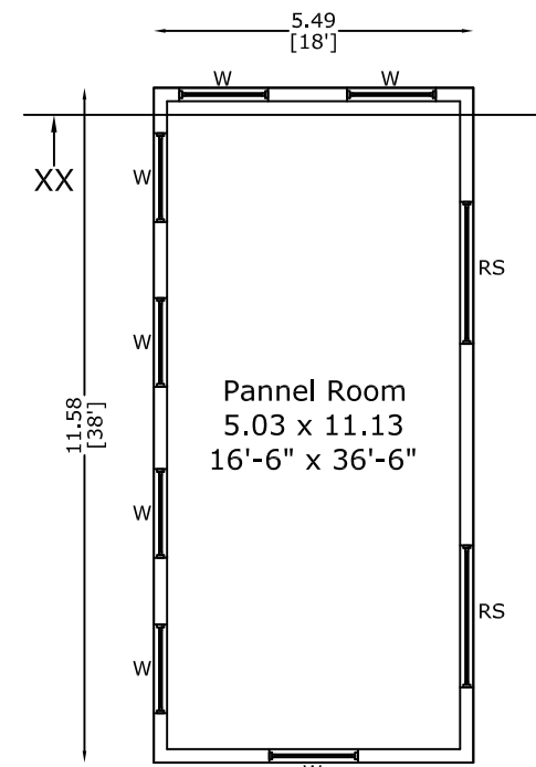
PANNEL ROOM
