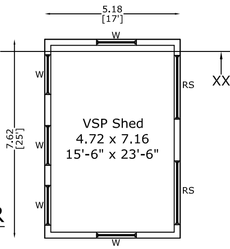
VSP SHED
