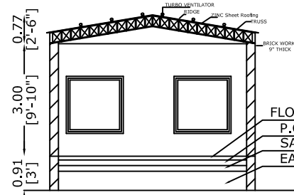
TYPICAL SECTION ON XX
