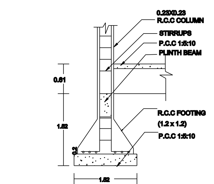
COLUMN DETAILS
