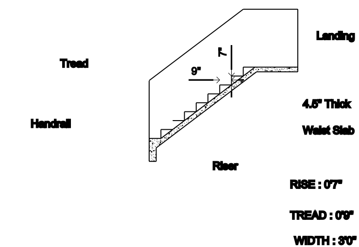
STAIRCASE DETAIL
