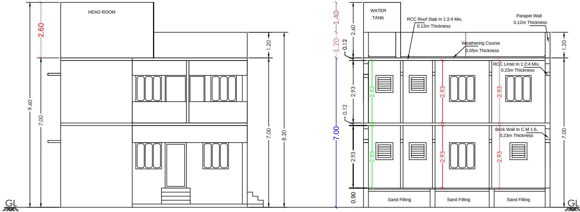
FRONT ELEVATION.
