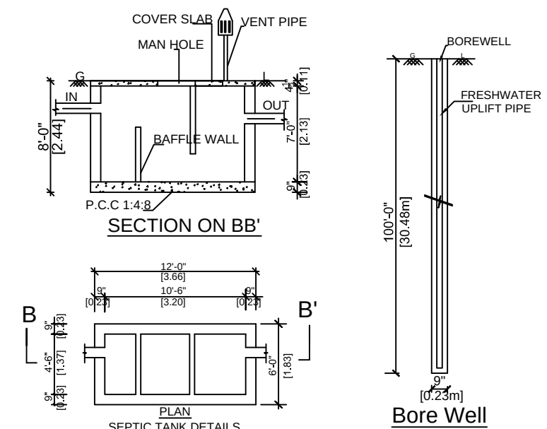
PLAN SEPTIC TANK DETAILS
