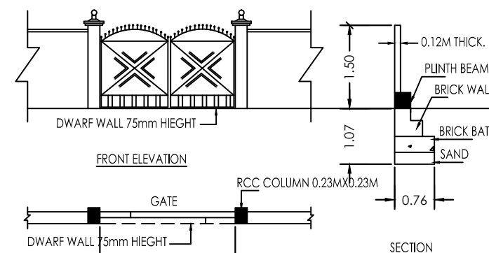
SECTION
