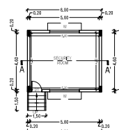
GROUND FLOOR PLAN
