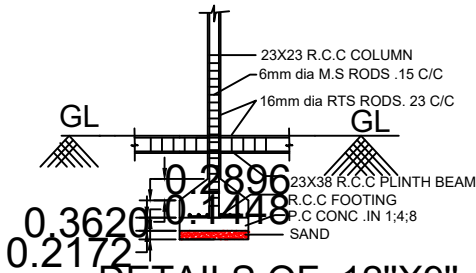
DETAILS OF .12"X9" COLOMN FOUNDATION
