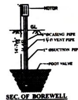
SEC. OF BOREWELL
