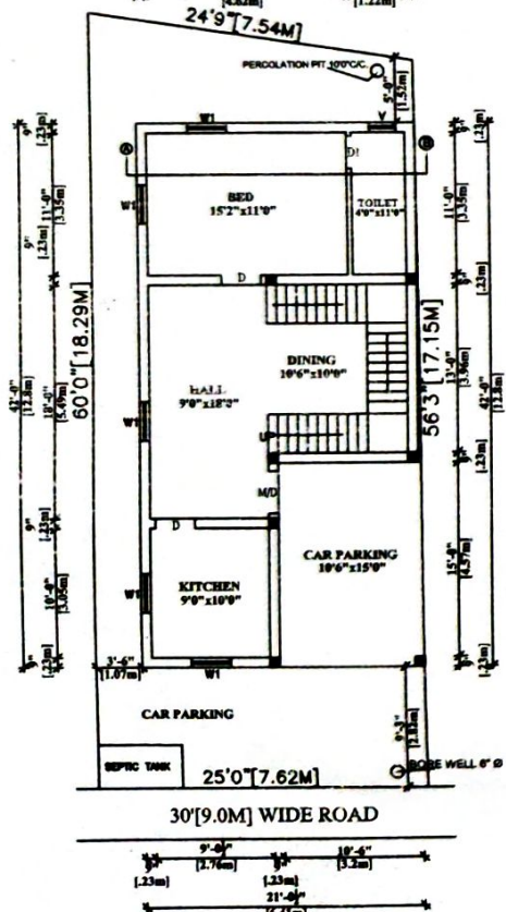
SITE CUM GROUND FLOOR PLAN
