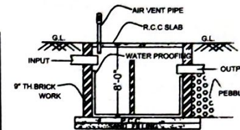
SECTION AT XX
