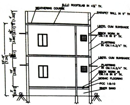
SECTION "AB"
