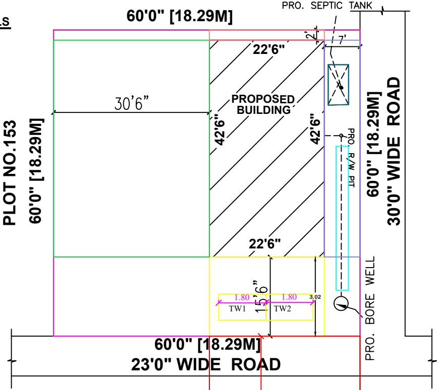
SITE PLAN
