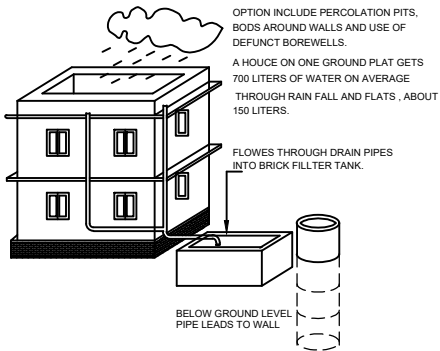
PERCULATION PIT
