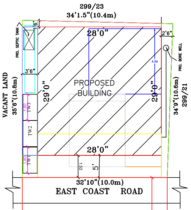
SITE PLAN
