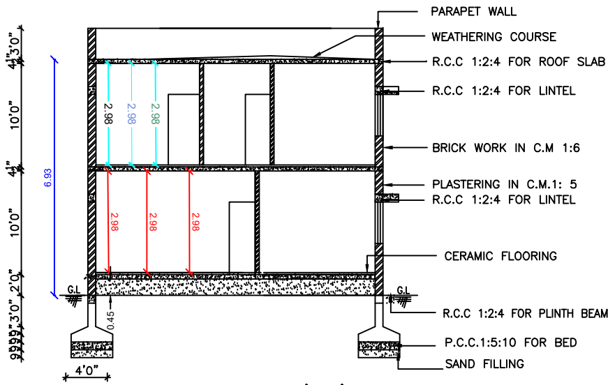
SECTION ON 'LS'
