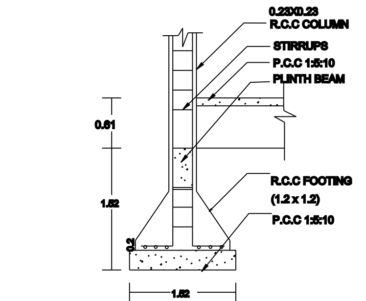
COLUMN DETAILS
