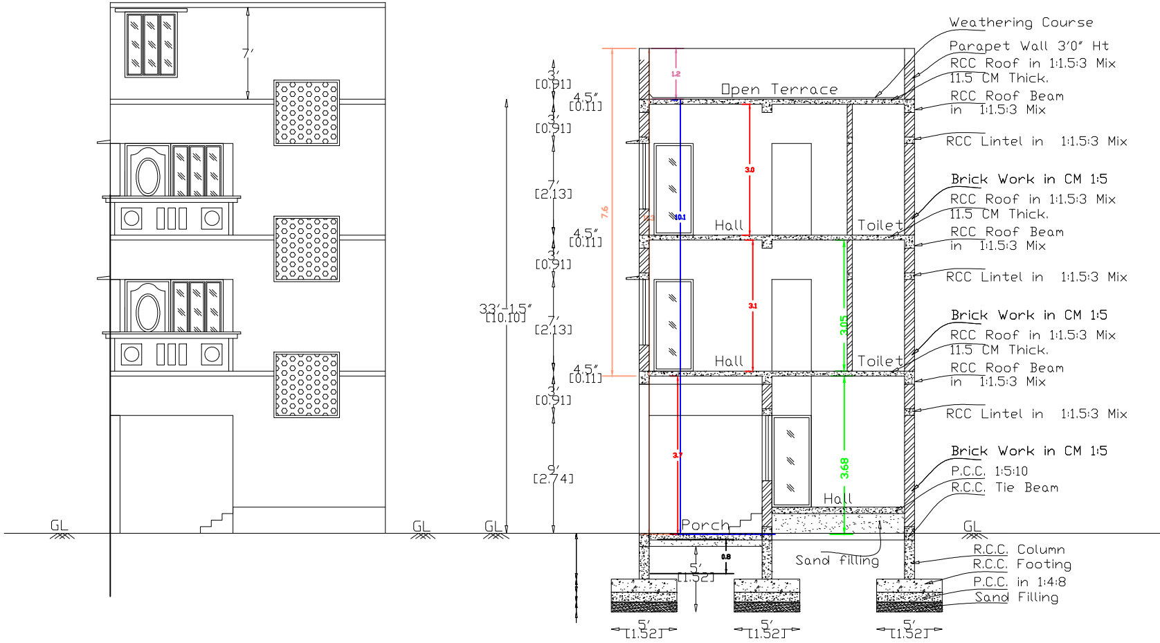
FRONT ELEVATION
