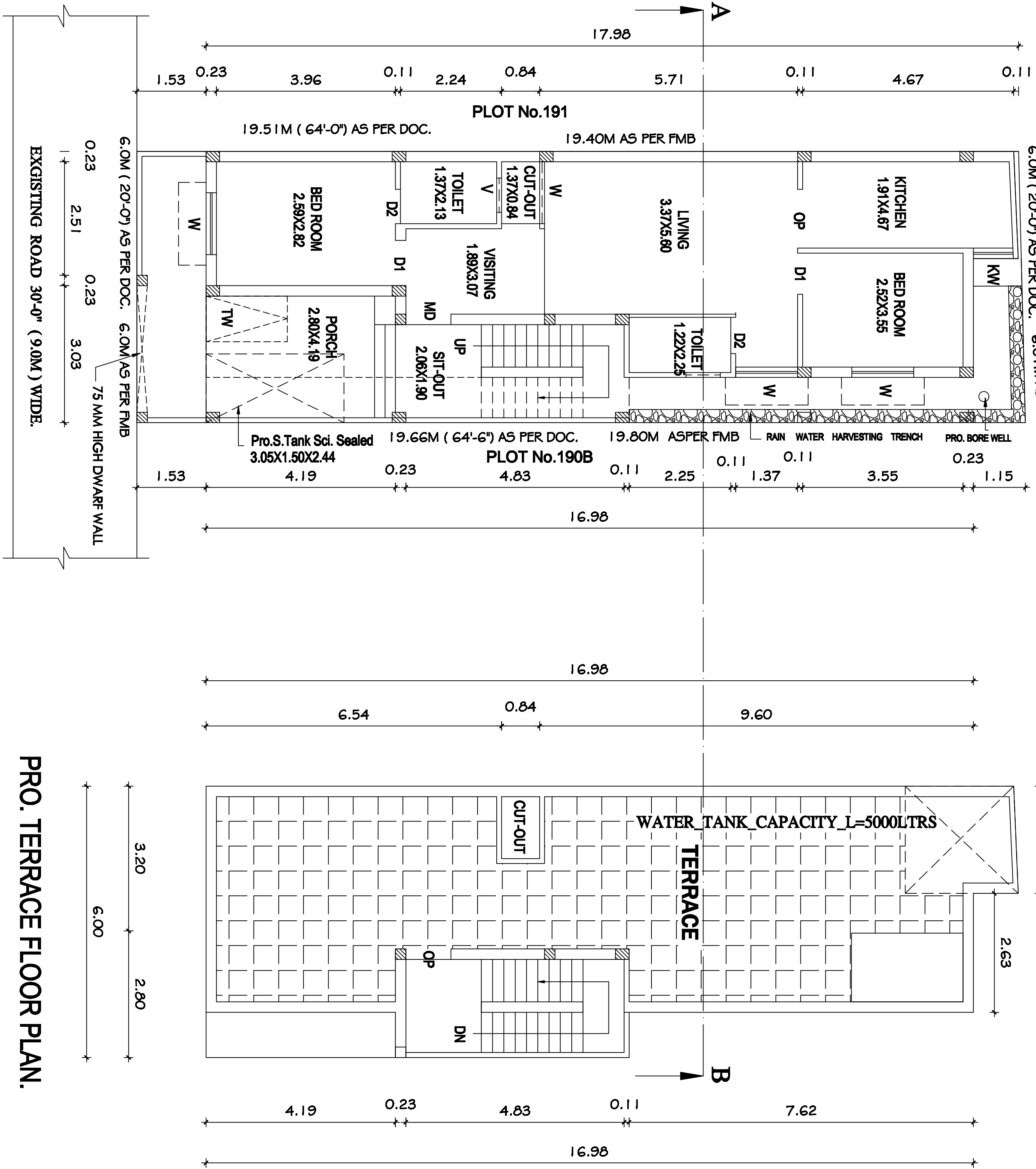
SITE cum PRO. GROUND FLOOR PLAN.
