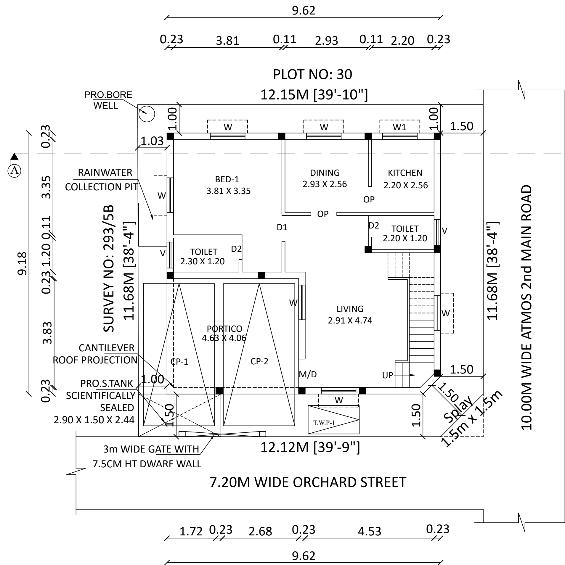
SITE CUM PRO.GROUND FLOOR PLAN
