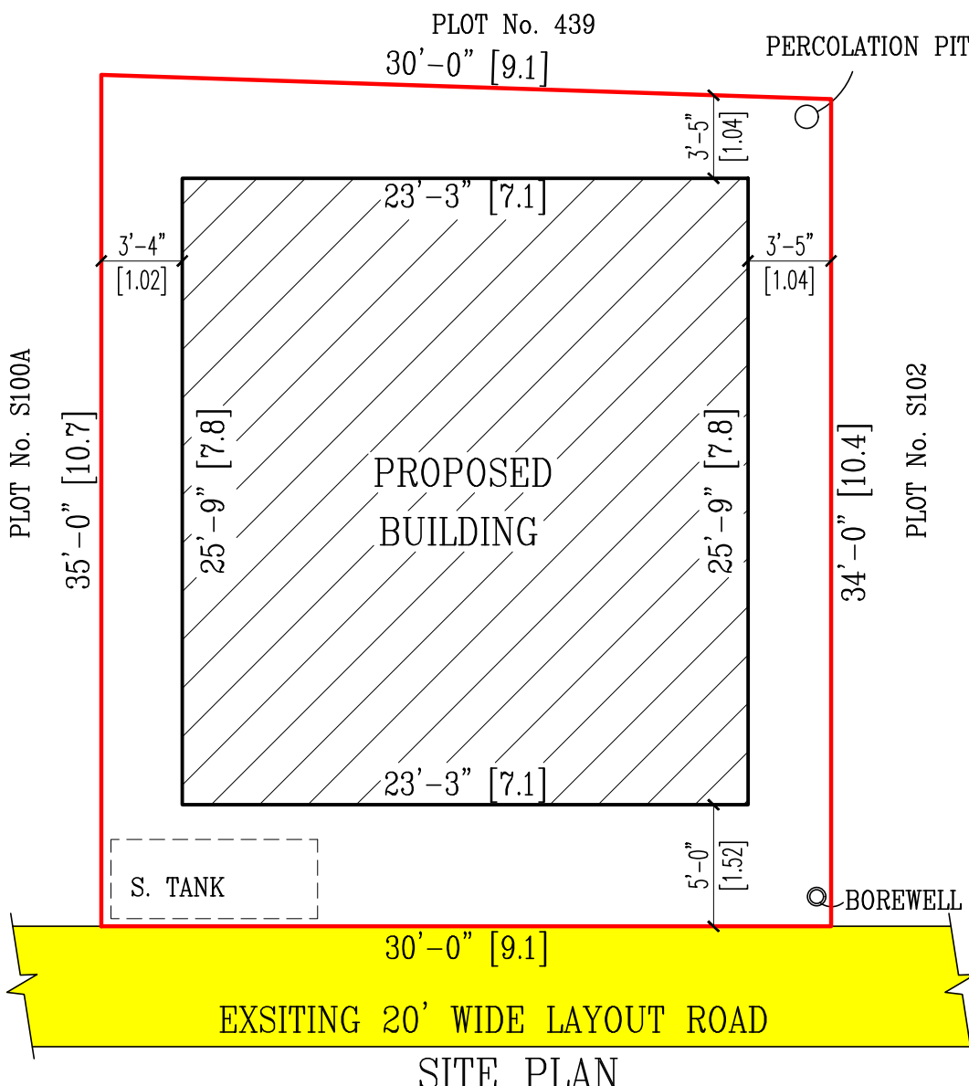
SITE PLAN
