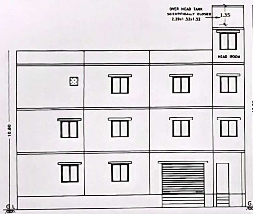
ELEVATION (PROPOSED)
