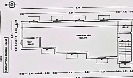
FIRST FLOOR PLAN (PROPOSED)
