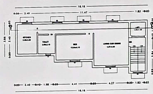
SECOND FLOOR PLAN (PROPOSED)
