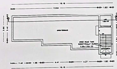
TERRACE FLOOR PLAN (PROPOSED)
