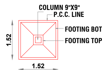
PLAN OF FOOTING
