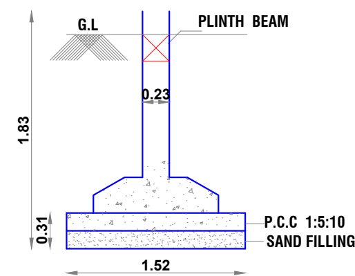
FOUNDATION DETAIL
