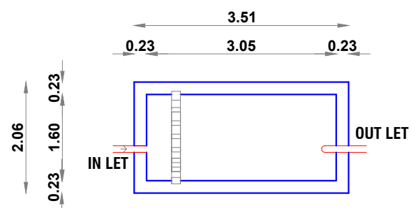
PLAN OF SEPTIC TANK CAPACITY - 8000 LITRES
