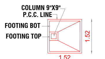
PLAN OF FOOTING
