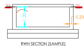
RWH_CAPACITY_L=5000LTRS
