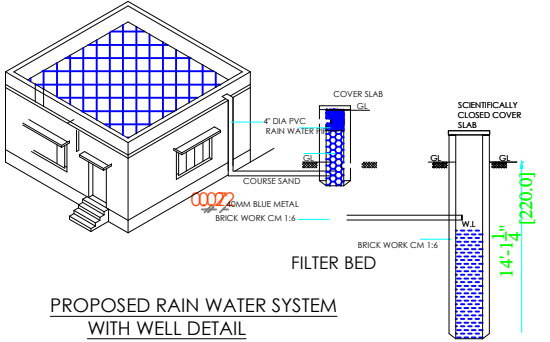
CROSS SECTION OF WELL 4'0" DIA
