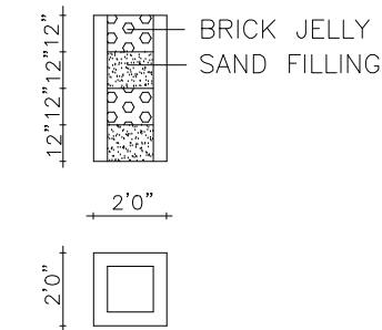
PERCOLATION PIT
