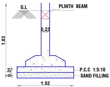
FOUNDATION DETAIL
