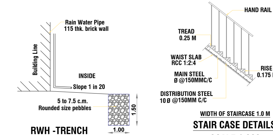
RWHTrench
