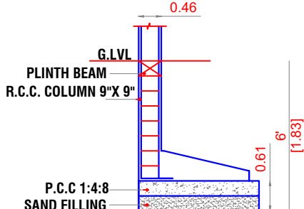
END FOOTING DETAILS
