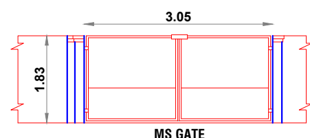
ELEVATION OF COMPOUND WALL
