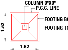
PLAN OF FOOTING
