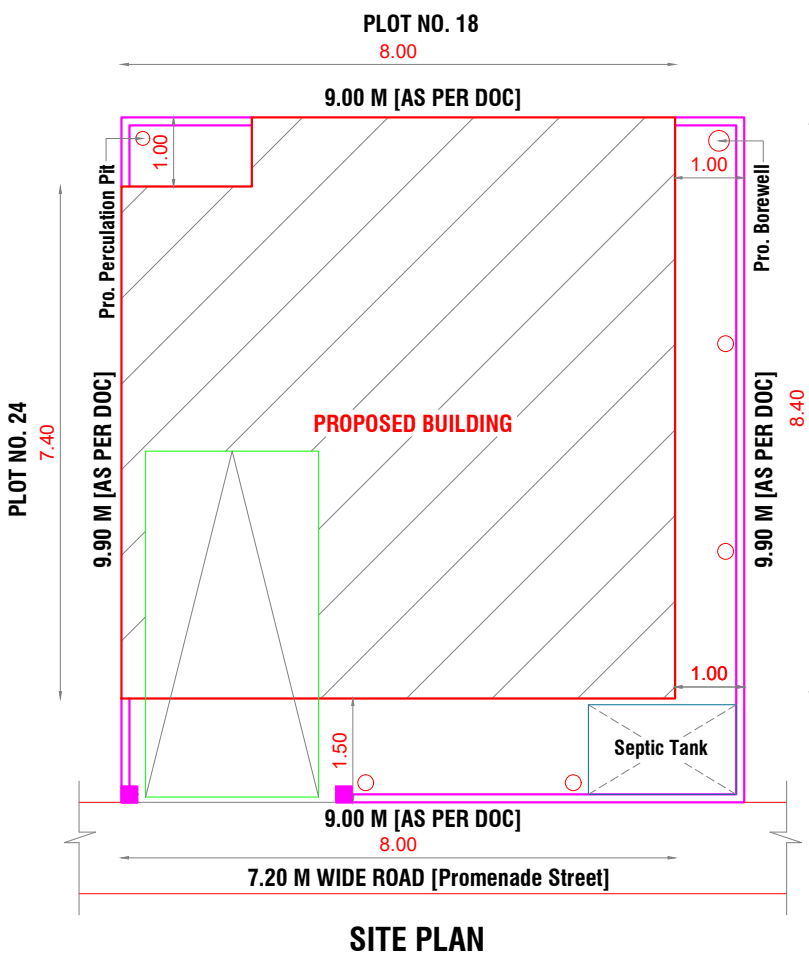
SITE PLAN
