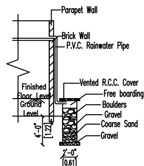
SECTION OF RAINWATER HARVESTING SYSTEM
