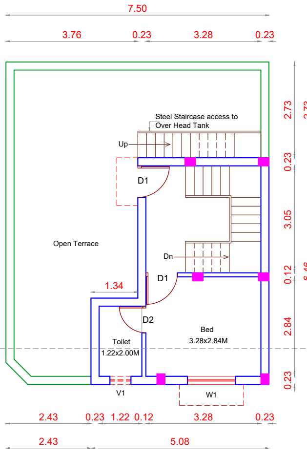
SECOND FLOOR PLAN [ PART ]
