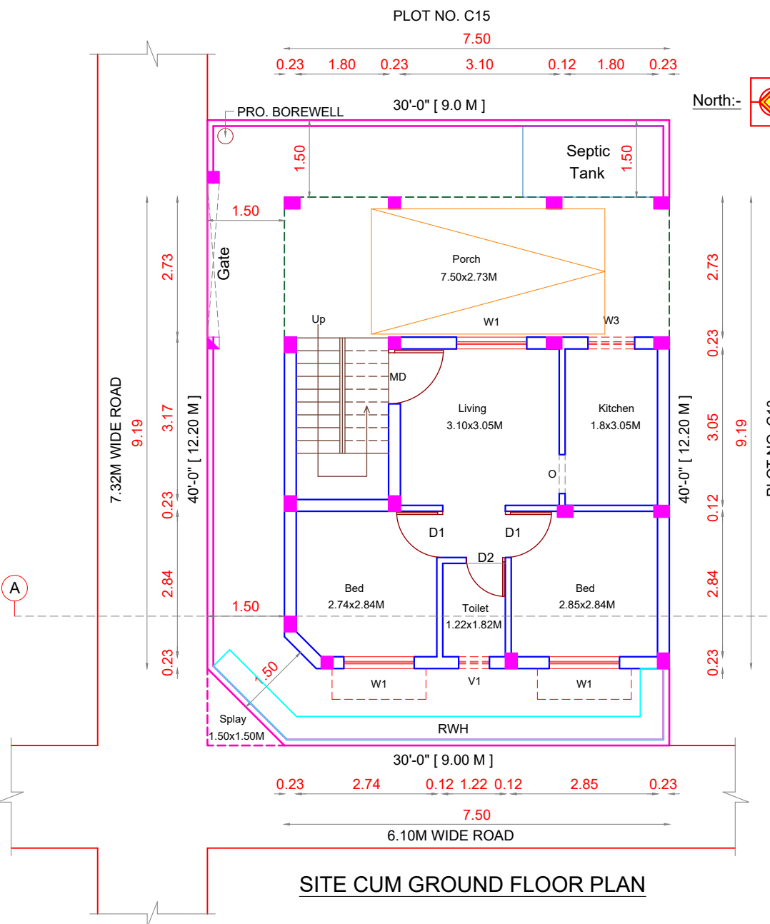
RWHTRENCH
