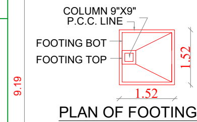
PLAN OF FOOTING
