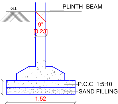
FOUNDATION DETAIL
