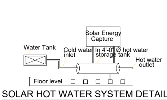
SOLAR HOT WATER SYSTEM DETAIL
