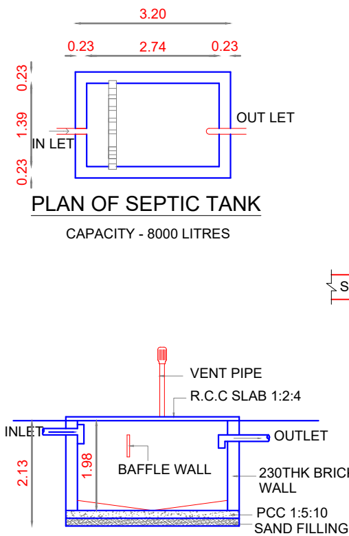
SECTION OF SEPTIC TANK
