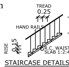
STAIRCASE DETAILS
