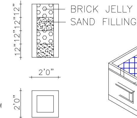
PERCOLATION PIT
