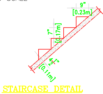
STAIRCASE DETAIL
